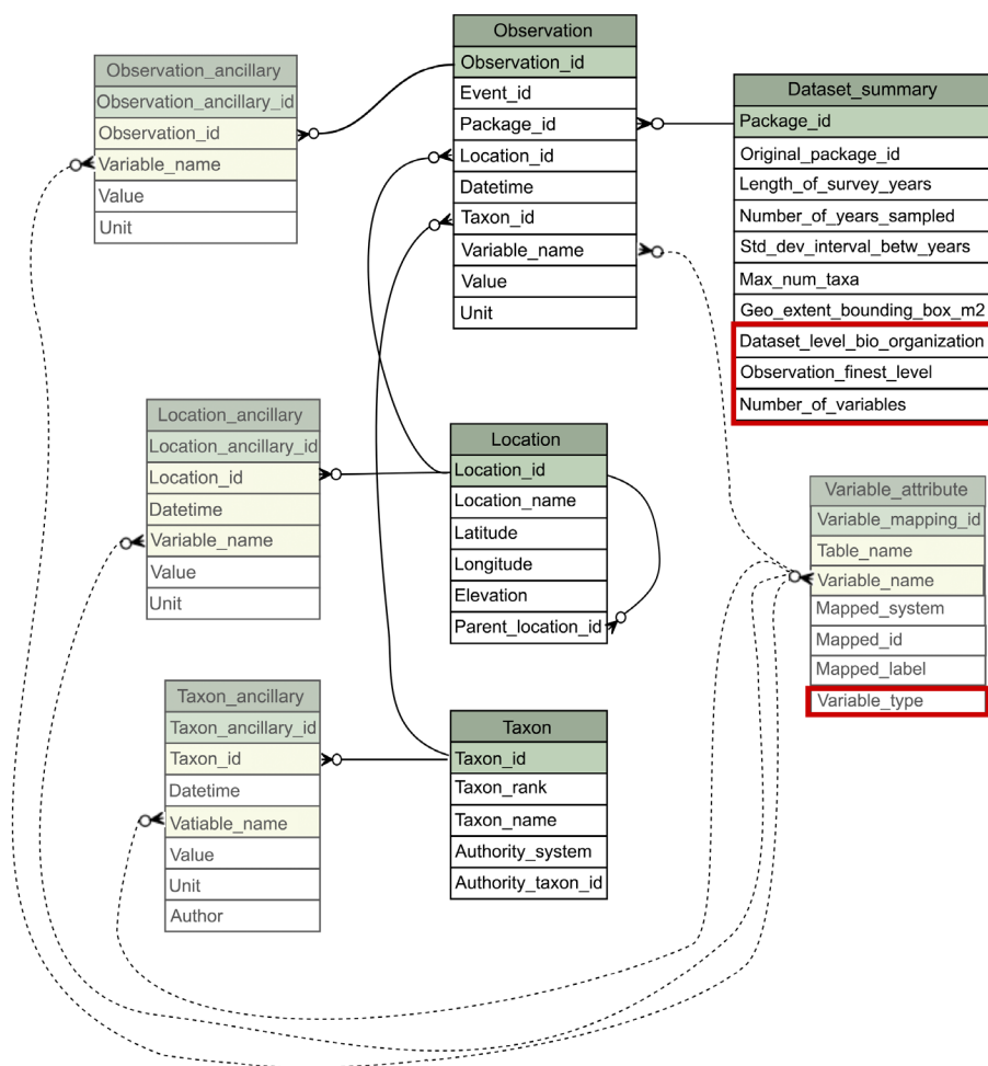
Fig. 4 Schema of the updated ecocomDP data design pattern with the extension to accommodate traits (O'Brien et al. , 2021). Added fields in the dataset summary table (boxed in red) allow users to include the level of biological organization, level of observation, and the number of variables associated with the trait. The variable attribute (previously variable_mapping) now includes variable type to indicate the type of trait measured (e.g. start and end dates).
