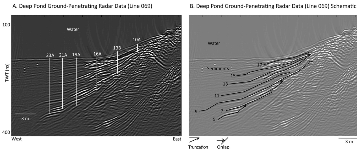
Fig. 2. A) Ground-penetrating radar profile moving from the center of the basin (left) towards the east shore (right) with two-way travel time (TWT) in nanoseconds along the y-axis and approximate position of core locations. B) Sedimentary features, such as onlaps and truncations, mapped onto the GPR profile. Numbers represent lowstands mentioned in the lake-level results.
