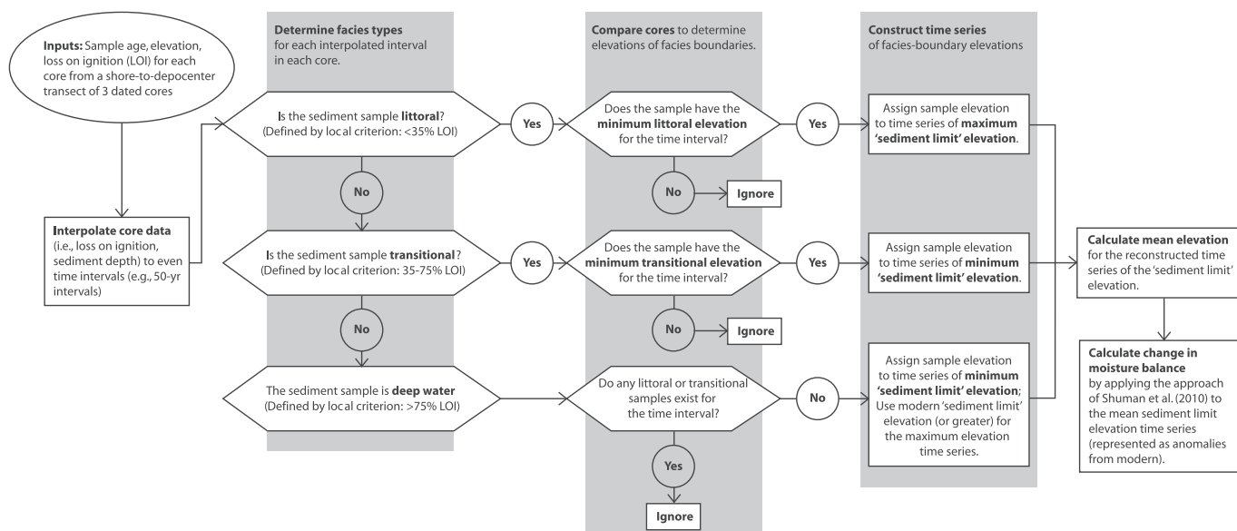
Fig. 3. Flow chart showing decision-tree approach to quantitatively reconstructing lake levels.
