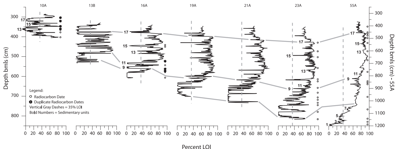
Fig. 6. Loss-on-ignition data for all cores in the transect plotted as depth below the modern lake surface (bmls). Open circles represent depths of radiocarbon ages. Gray lines track major stratigraphic boundaries, and low LOI intervals associated with lowstands are labeled by the unit numbers mentioned in the text (e.g., 13, 15, 17, etc.).
