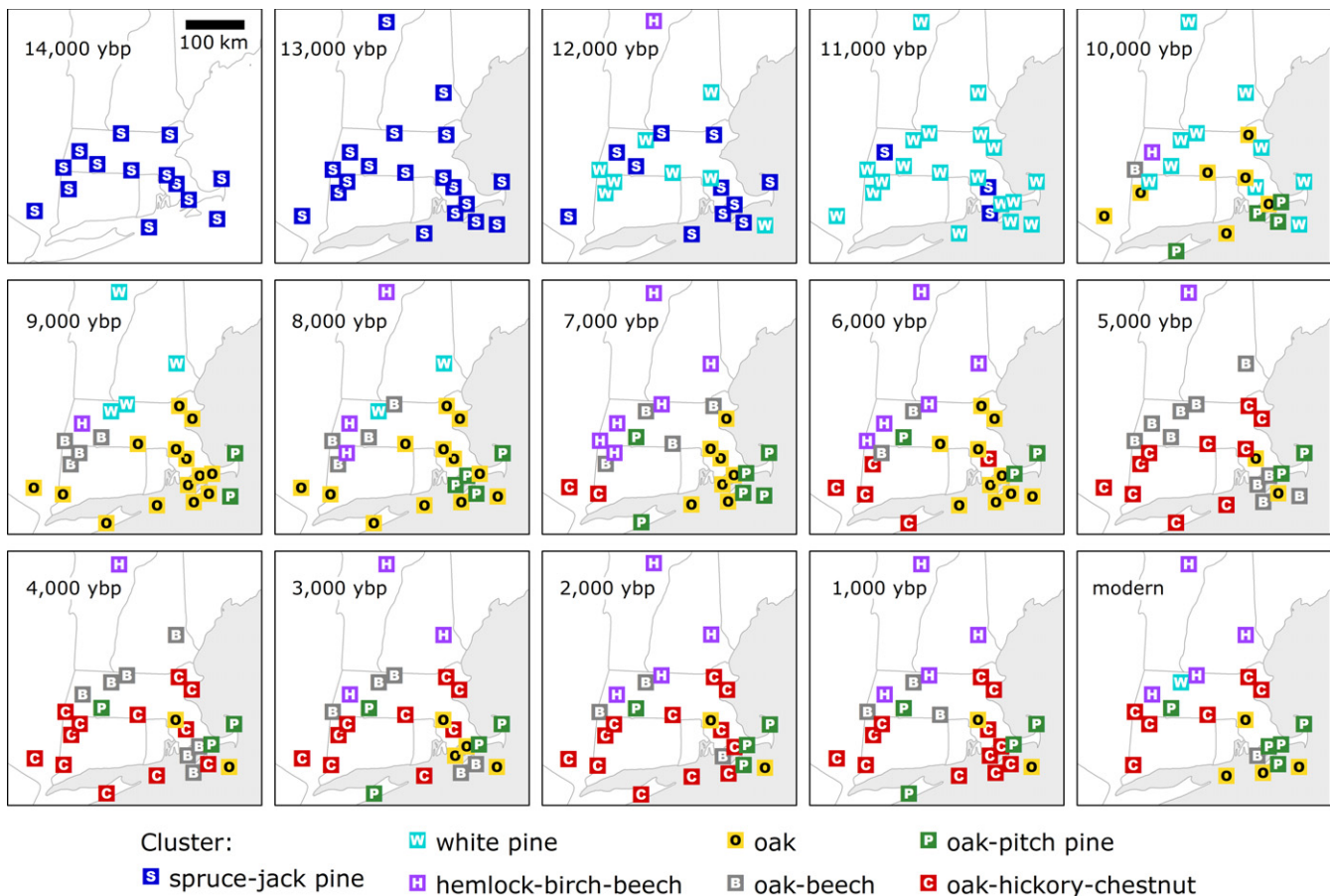
FIGURE 4 Results of cluster analysis of pollen percentage data from New England lake-sediment pollen records; cluster assignments mapped at 1,000-year intervals [Colour figure can be viewed at wileyonlinelibrary.com ]
