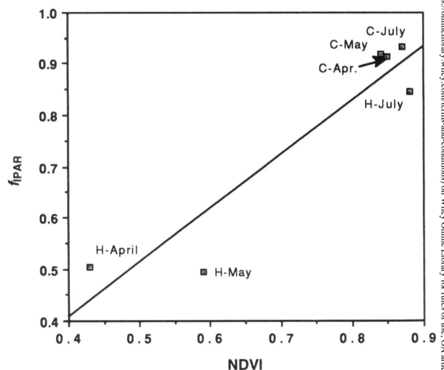
Figure 2. The normalized difference vegetation index (NDVI) determined over areas dominated by conifers (C) and deciduous hardwoods (H) indicates that essentially all seasonal variation is attributed to the hardwood component. y = -0.01 + 1.050x ; R^2 = 0.88 . October estimates of NDVI of 0.61 for areas with pure hardwoods correspond to an equivalent fraction of PAR interception ( f_{IPAR} ) of 0.63. The actual f_{IPAR} value, however, was still > 0.8 under the predominantly hardwood canopy near the tower (Fig. 1), indicating that NDVI integrates chlorophyll content as well as leaf area index (Table 3).
