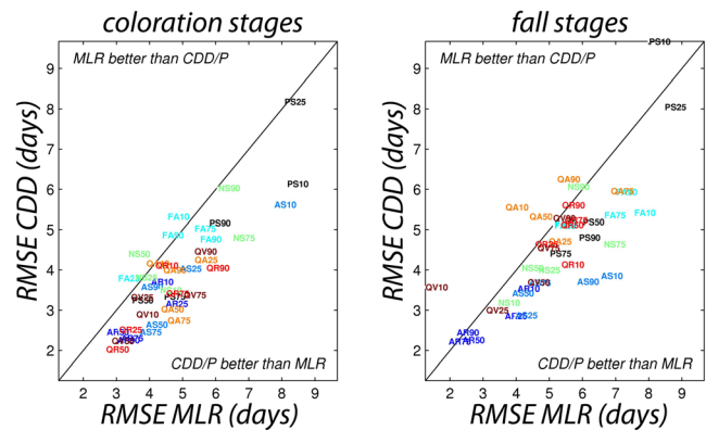
Figure 4. Comparison of the empirical and process-oriented models. Comparison of goodness-of-fit (in terms of RMSE) of empirical (MLR) and process-oriented (CDD/P) models for leaf coloration (left) and leaf fall (right), in a leave-one-out cross-validation analysis. The MLR model is shown to be less robust, as its RMSE is higher (to the right of the 1:1 line) in a majority of cases. doi:10.1371/journal.pone.0057373.g004
