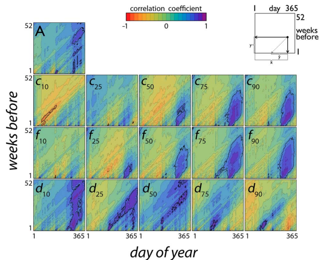
Figure 3. Correlation between interannual variation in temperature and interannual variation in autumn color phenology in red maple, Acer rubrum . Each point (x,y) in each plot represents a time window spanning the y weeks (vertical axis) before day x (horizontal axis). The color at each point (x,y) represents the correlation between the average air temperature for the time window (x,y) and the measure of autumn leaf phenology for that plot: onset of autumn colors ( c_x ), time of leaf fall ( f_x ), duration of autumn colors ( d_x ) and total amount of color (A). Values of R are shown by colors ranging from orange-red (minimum, negative) to blue-purple (maximum, positive); absolute values of R > 0.468 (the critical value of the Pearson product-moment correlation coefficient; p = 0.05 ; d.f. = 16 ) are inside the bold lines. Here, both leaf fall and the display of red leaves were shifted significantly later in years with warmer autumn temperatures. Dates of the full display of autumn colors ( c_{75} , c_{90} ) were positively correlated with temperatures from spring through (especially) autumn, while warmer spring temperatures are correlated with earlier onset of color ( c_{10} ). Both the duration of autumn colors ( d_x ) and the total amount of autumn color (A) tended to increase in years with warmer temperatures. doi:10.1371/journal.pone.0057373.g003
