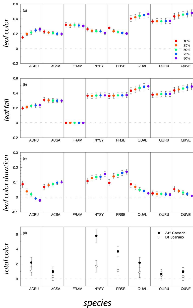
Figure 5. Projected rates of change in the timing of leaf coloration and leaf fall (5a and 5b; dates at which thresholds of 10%, 25%, 50%, 75% and 90% were reached), leaf color duration (5c; number of days between different leaf color duration thresholds and 90% leaf fall), and total amount of autumn colors (5d). For each species, the process-oriented (CDD/P) model, calibrated to 18 years of field data, was run forward using statistically downscaled climate projections from the GFDL CM2 model (IPCC A1fi and B1 scenarios; only A1fi scenario results shown in panels a through c). Projected rates of change (as plotted on the y-axis) were then calculated as the slope of the linear regression line between each phenological variable and year, over the period 2010–2099. Thus, for panels a through c, units are days per year, whereas for d, units are amount of color/year. ACRU: Acer rubrum ; ACSA: Acer saccharum ; FRAM: Fraxinus americana ; NYSY: Nyssa sylvatica ; PRSE: Prunus serotina ; QUAL: Quercus alba ; QURU: Quercus rubra ; QUVE: Quercus velutina . doi:10.1371/journal.pone.0057373.g005
