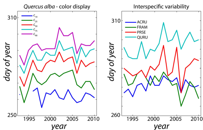
Figure 2. Interannual variability of autumn senescence stages. 2a: timing of leaf coloration stages ( c_{10} =10% of leaves colored ... c_{90} =90% of leaves coloured) for Quercus alba , white oak. 2b: timing of 50% leaf fall for four species (ACRU = Acer rubrum ; FRAM = Fraxinus americana , PRSE = Prunus serotina ; QURU = Quercus rubra ). doi:10.1371/journal.pone.0057373.g002
