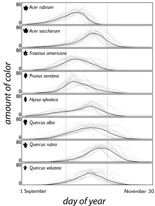
Figure 1. The amount of autumn colors over time for eight deciduous broadleaf species that turn red in autumn. The amount of autumn color (0–100) is calculated as i_n(100 - j_n) on day n , where the percentage of red leaves i_n is multiplied by the percentage of leaves retained ( 100 - j_n ). Individual years (1993–2010) are shown by dotted lines, and their average by the thick curve. doi:10.1371/journal.pone.0057373.g001
