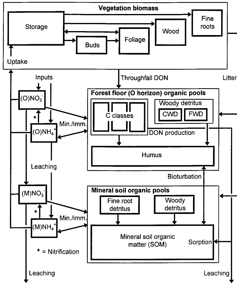
FIG. 1. Schematic of the hierarchical structure of pools and fluxes of nitrogen in TRACE 2.1. Plant uptake of N, detrital N dynamics, and N transformations are calculated separately in each soil layer. Pools of KCl-extractable N are separated by soil layer: (O) = O horizon, (M) = mineral soil. DON = dissolved organic nitrogen. CWD, FWD = coarse and fine woody detritus. Min./imm. = Mineralization and assimilation. Inputs = NO_3^- and NH_4^+ in atmospheric deposition, fertilizer, and isotopic tracer additions. For clarity, not all fluxes are shown in detail.
