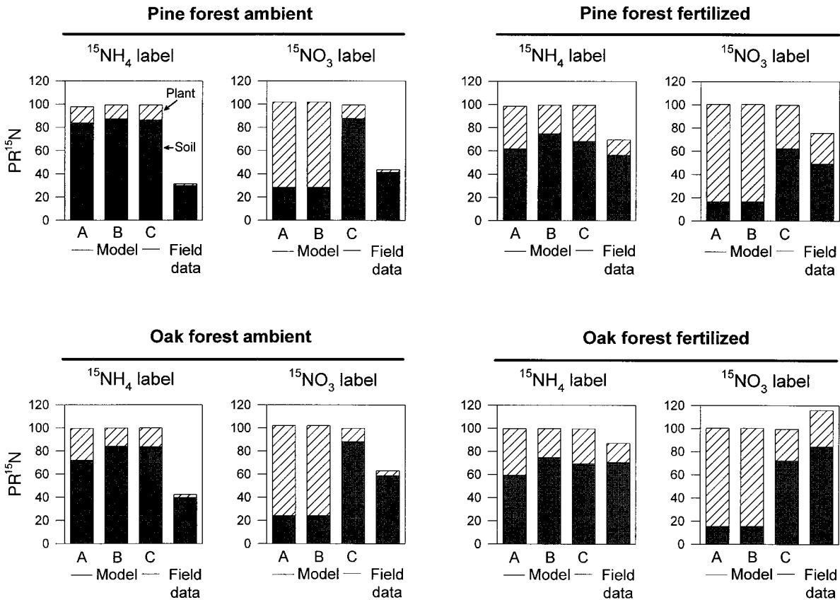
FIG. 4. Percent recovery ( PR^{15}N ) for total mass of ^{15}N tracers at the end of tracer applications, which spanned two growing seasons. Hatched bars = sum of plant pools; solid bars = sum of soil pools. Three iterations of model predictions are shown (indicated by A, B, C; described in Table 2). Field data are from Nadelhoffer et al. (1999).
