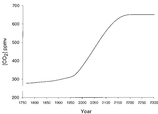
Fig. 1. Atmospheric CO 2 concentration from 1765 to 2300 as prescribed by the IPCC S650 concentration profile.
